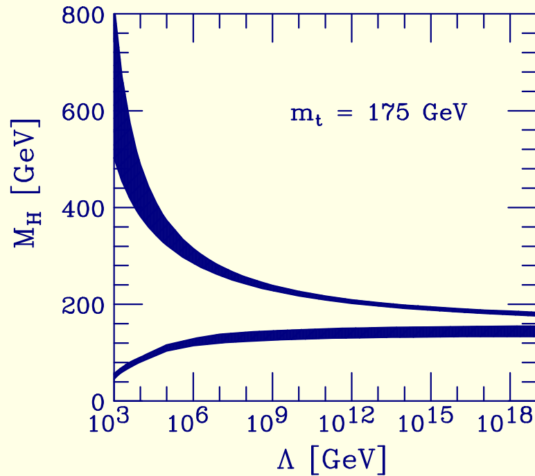
Figure 2: Left: triviality and global minimum constraints on m_{h_{SM}} vs. \Lambda . Right: fine-tuning constraints on \Lambda .
