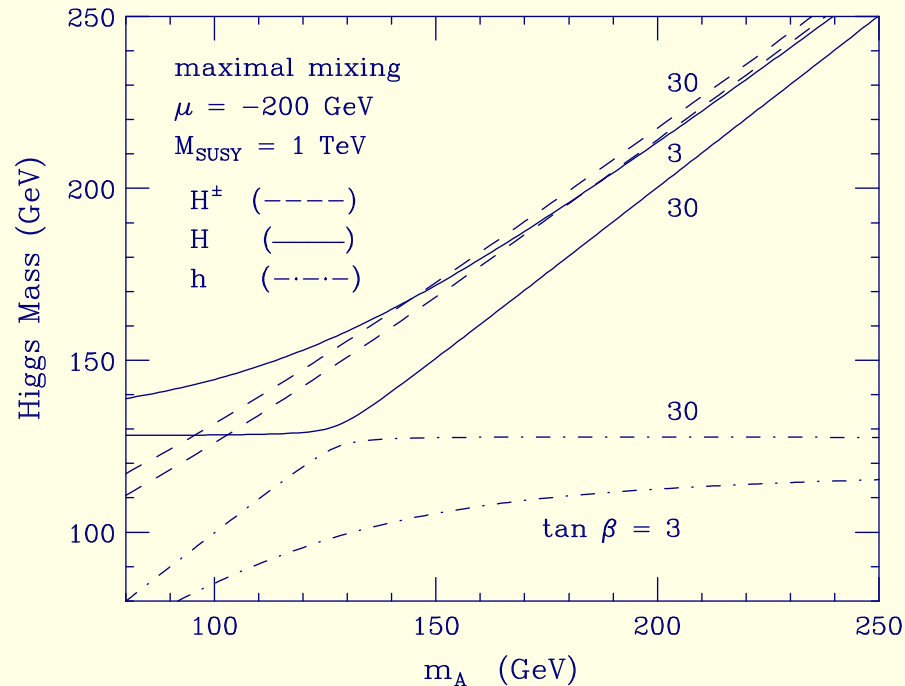
Figure 10: Higgs masses as a function of m_{A^0} for maximal mixing with m_{\text{SUSY}} = M_Q = M_U = M_D = 1 TeV.
