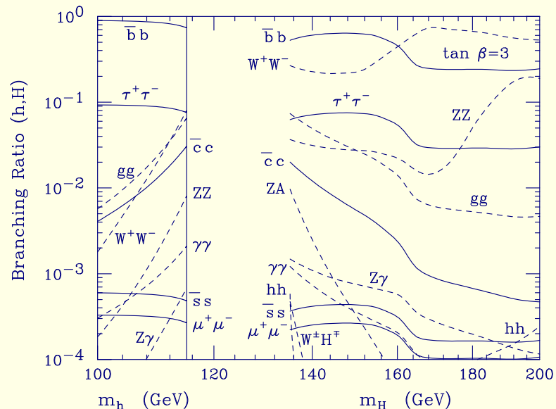
Figure 15: Branching ratios for h^0 and H^0 at lower mass.
