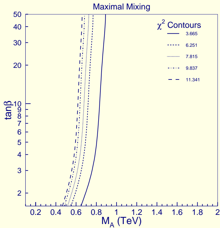
Figure 23: Contours of \chi^2 for Higgs boson decay observables for (a) the maximal mixing scenario; and (b) a choice of MSSM parameters for which the loop-corrected h^0 b \bar{b} coupling is suppressed large \tan \beta and low m_{A^0} . Results are based on Higgs measurements anticipated at the LC with \sqrt{s} = 500 GeV and L = 500 fb^{-1} . The contours correspond to 68, 90, 95, 98 and 99% confidence levels (right to left) for the observables g_{hbb}^2 , g_{h\tau\tau}^2 , and g_{hgg}^2 .
