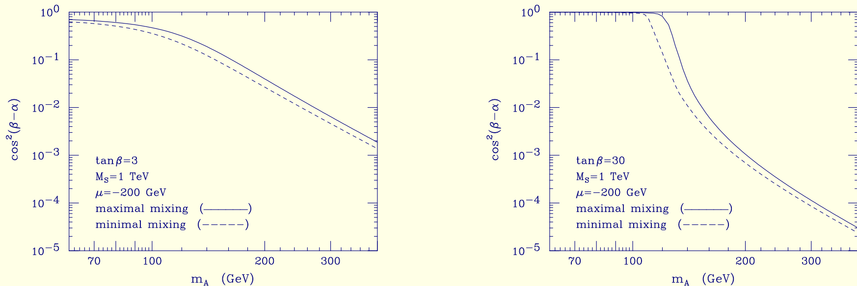
Figure 11: Minimal and maximal mixing results for approach to decoupling.
