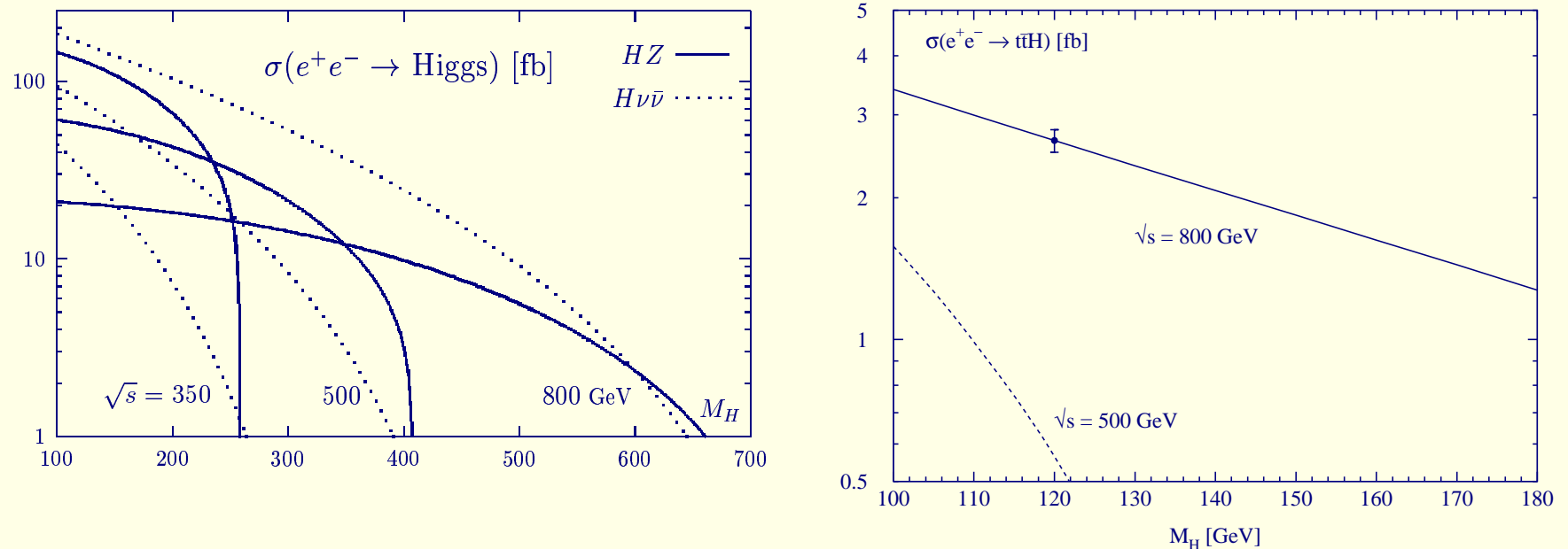
Figure 7: SM Higgs \sigma 's at the LC. Recall: L = 200 - 300\text{fb}^{-1} per year.
