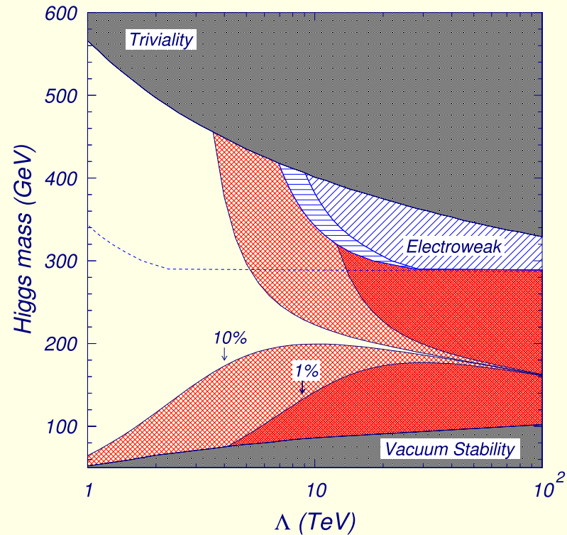
Figure 2: Left: triviality and global minimum constraints on m_{h_{SM}} vs. \Lambda . Right: fine-tuning constraints on \Lambda .
