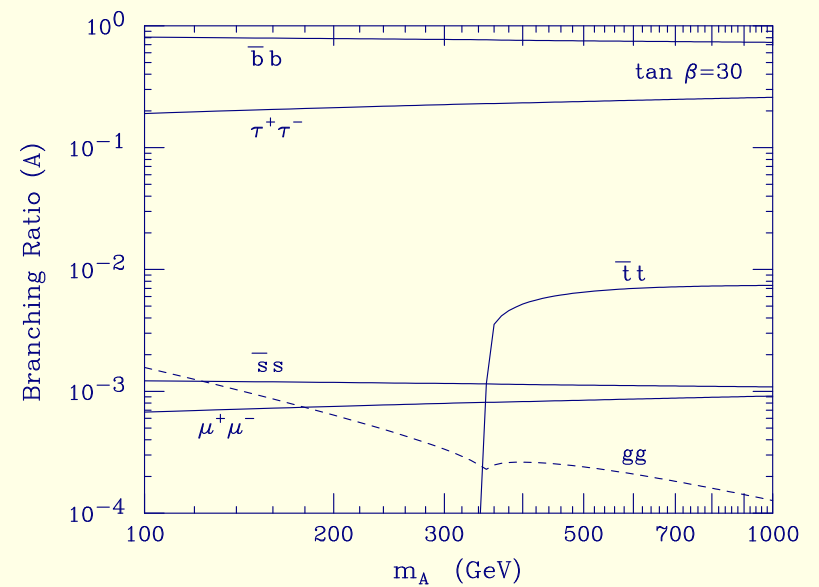
Figure 13: Branching ratios for A^0 .
