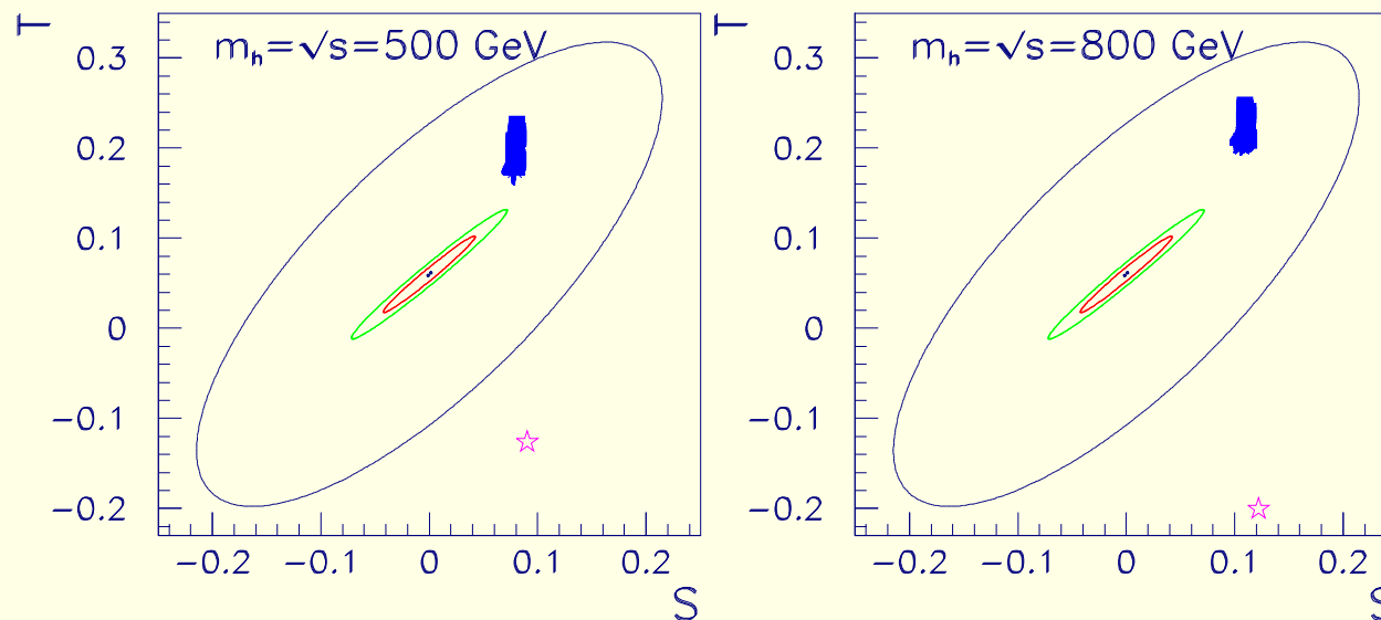
Figure 3: Outer ellipses = current 90% CL region for U = 0 and m_{h_{\text{SM}}} = 115 \text{ GeV} . Blobs = S, T predictions for Yukawa-wedge 2HDM models with minimum relative \Delta\chi^2 . Innermost (middle) ellipse = 90% (99.9%) CL region for m_{h_{\text{SM}}} = 115 \text{ GeV} after Giga- Z and a \Delta m_W \lesssim 6 \text{ MeV} threshold scan measurement. Stars = SM S, T prediction if m_{h_{\text{SM}}} = 500 or 800 \text{ GeV} .
