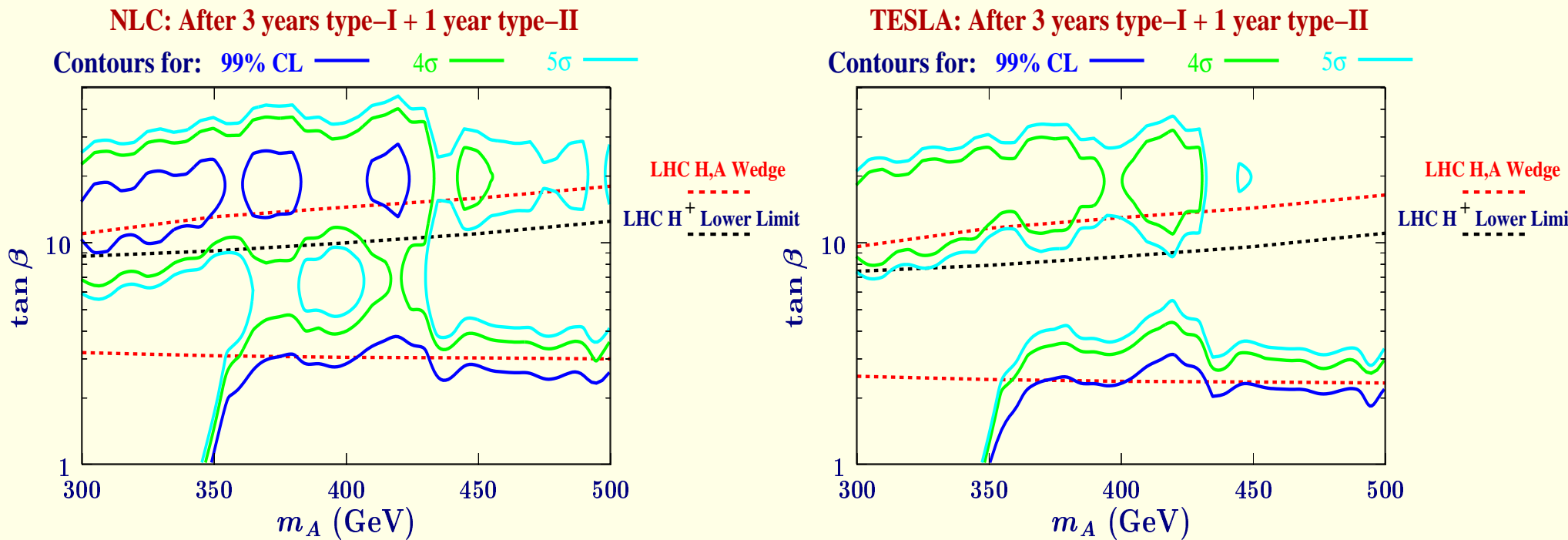
Figure 22: Contours for discovery and 99% CL exclusion after 4 years of NLC or TESLA \gamma\gamma running. (Ignore the H^+ wedge line — it has moved up above the H^0, A^0 line.)
