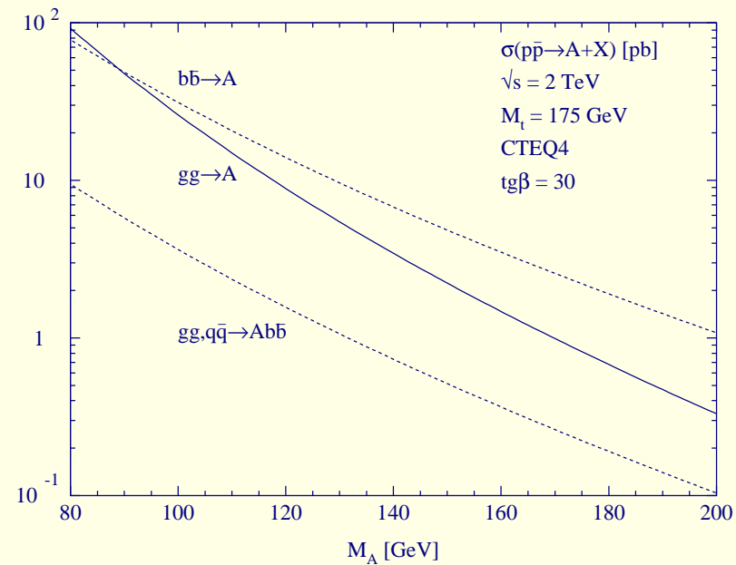
Figure 18: Tevatron cross sections.
