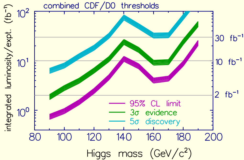
Figure 6: SM Higgs discovery at Tevatron and LHC. h_{\text{SM}} detection is guaranteed at the LHC.
