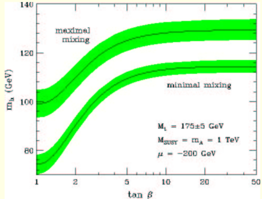
Figure 8: Left: m_{h^0} as function of X_t . Right: m_{h^0} as a function of \tan\beta for X_t = 0 (minimal mixing) and X_t = \sqrt{6}M_S (maximal mixing). m_{\text{SUSY}} = M_Q = M_U = M_D .
