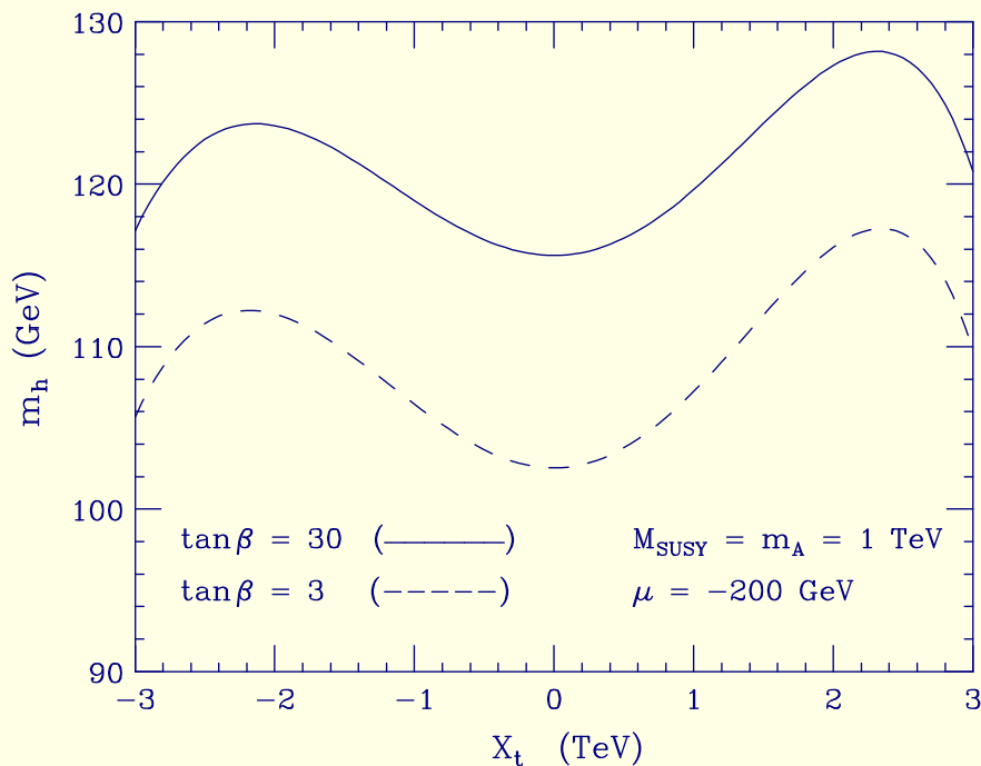
Figure 8: Left: m_{h^0} as function of X_t . Right: m_{h^0} as a function of \tan\beta for X_t = 0 (minimal mixing) and X_t = \sqrt{6}M_S (maximal mixing). m_{\text{SUSY}} = M_Q = M_U = M_D .
