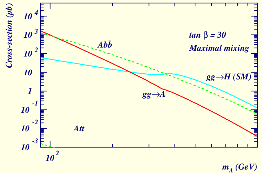
Figure 19: Neutral MSSM Higgs production cross-sections at the LHC. The cross section for gluon-gluon fusion to a SM Higgs boson is also shown.
