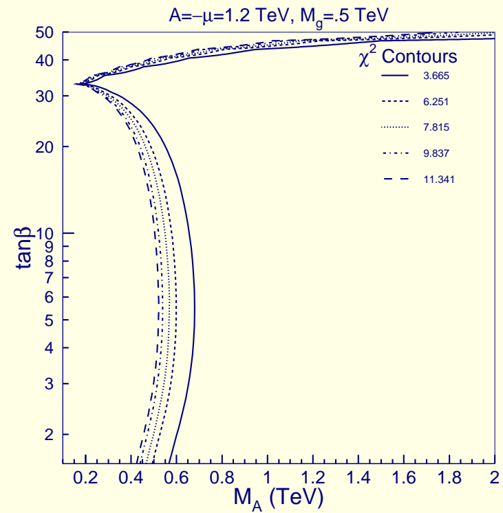
Figure 23: Contours of \chi^2 for Higgs boson decay observables for (a) the maximal mixing scenario; and (b) a choice of MSSM parameters for which the loop-corrected h^0 b \bar{b} coupling is suppressed large \tan \beta and low m_{A^0} . Results are based on Higgs measurements anticipated at the LC with \sqrt{s} = 500 GeV and L = 500 fb^{-1} . The contours correspond to 68, 90, 95, 98 and 99% confidence levels (right to left) for the observables g_{hbb}^2 , g_{h\tau\tau}^2 , and g_{hgg}^2 .
