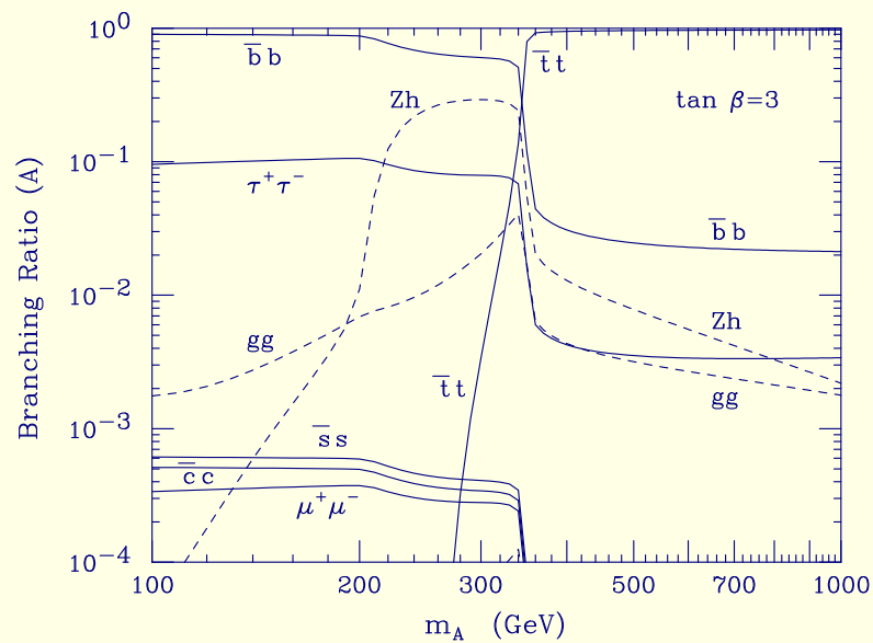
Figure 13: Branching ratios for A^0 .
