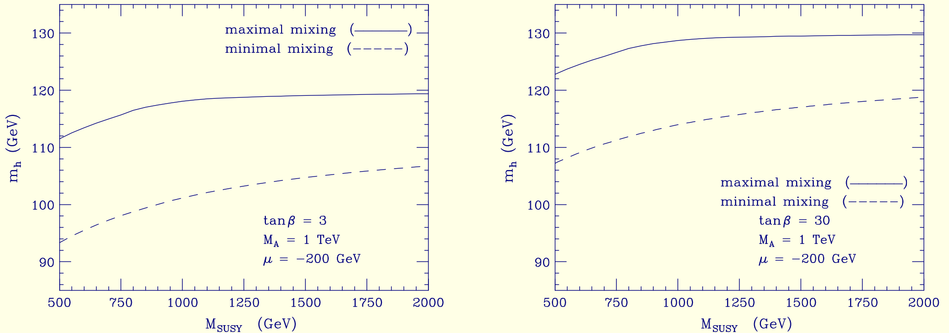
Figure 9: Minimal and maximal mixing results for m_{h^0} as a function of m_{\text{SUSY}} = M_Q = M_U = M_D .
