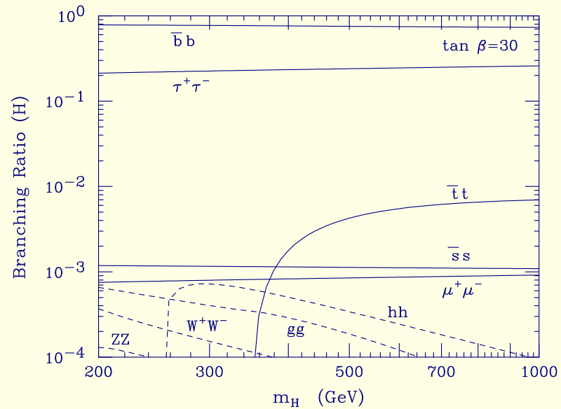
Figure 16: Branching ratios for H^0 to higher mass.
