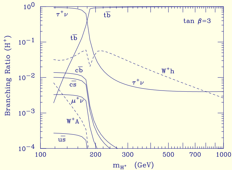
Figure 14: Branching ratios for H^\pm .
