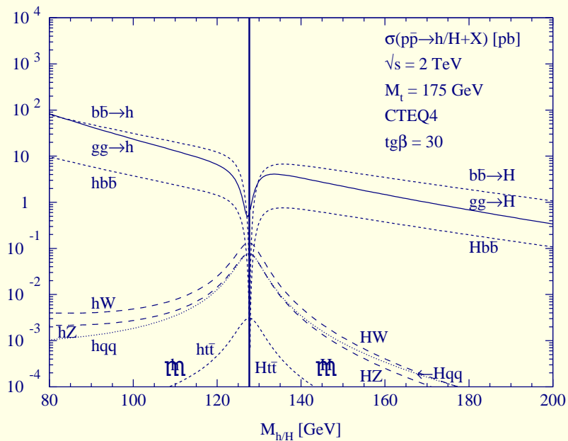
Figure 18: Tevatron cross sections.
