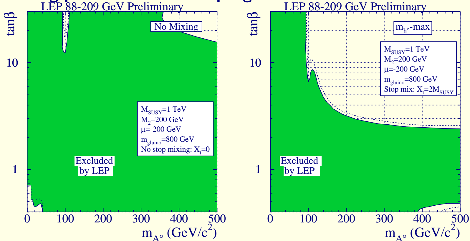
Figure 20: LEP2 limits for minimal and maximal mixing.
