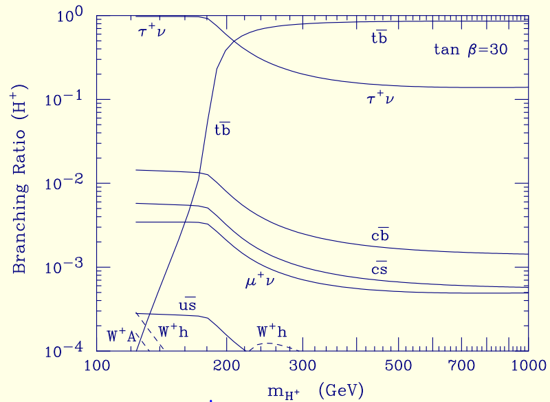
Figure 14: Branching ratios for H^\pm .
