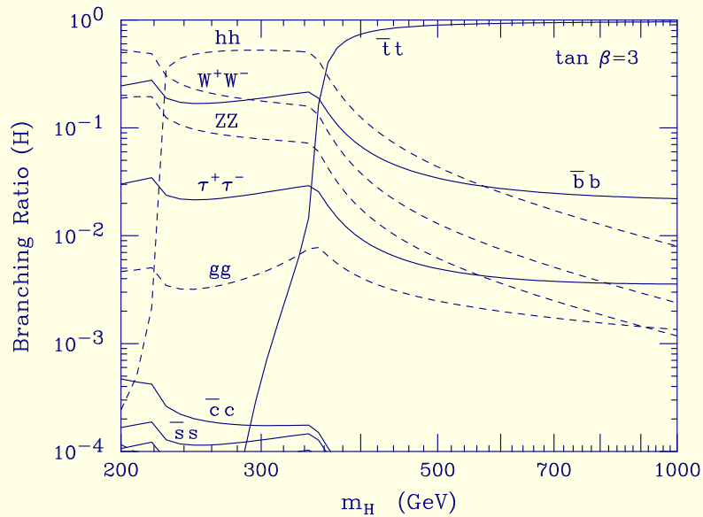
Figure 16: Branching ratios for H^0 to higher mass.
