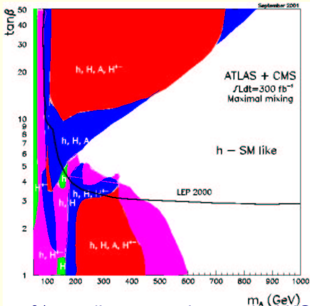
Figure 21: 5\sigma discovery regions at the LHC.
