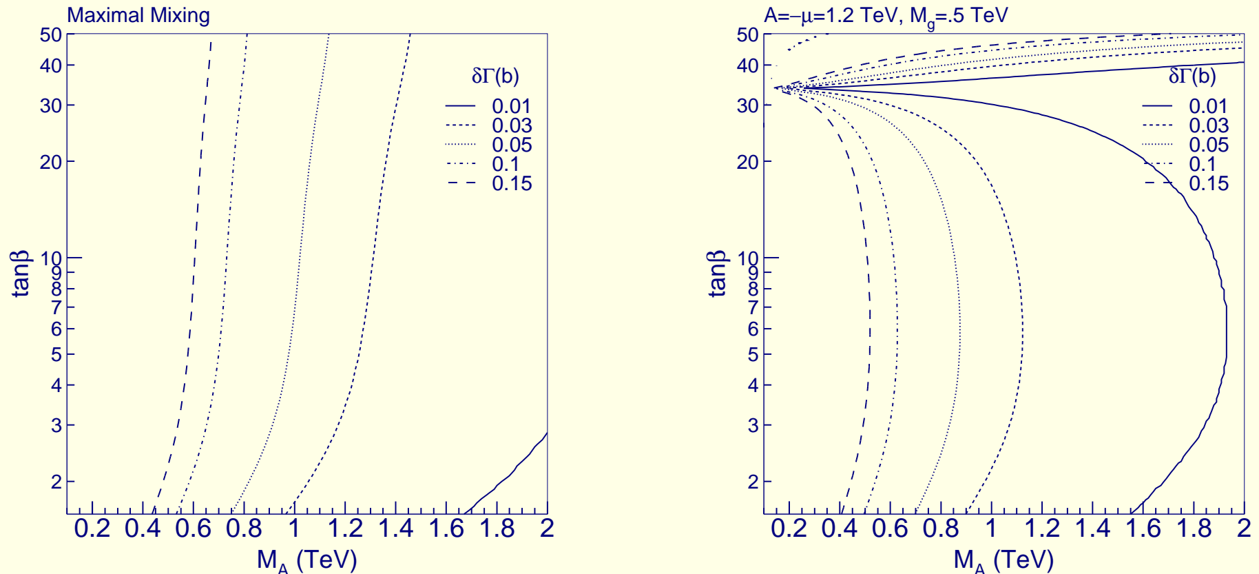
Figure 12: Deviations of \Gamma(h^0 \rightarrow b\bar{b}) relative to SM value for “normal” case and m_{A^0} -independent scenario.
