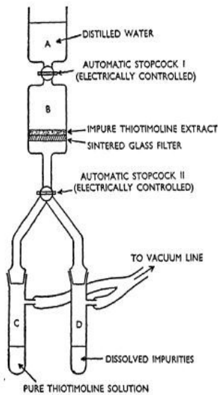
Figure 6. Simplified form of Endochronic filter.
